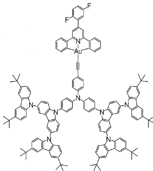
Compound 5
