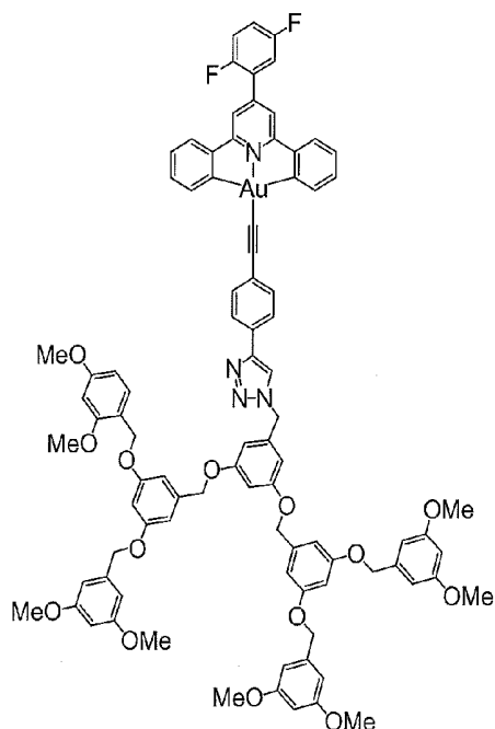
Compound 3
