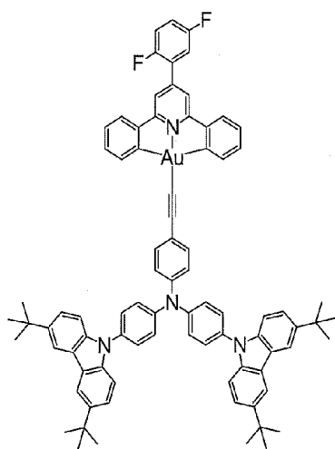
Compound 4
