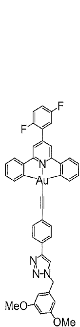
Compound 1
