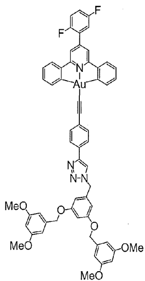
Compound 2
