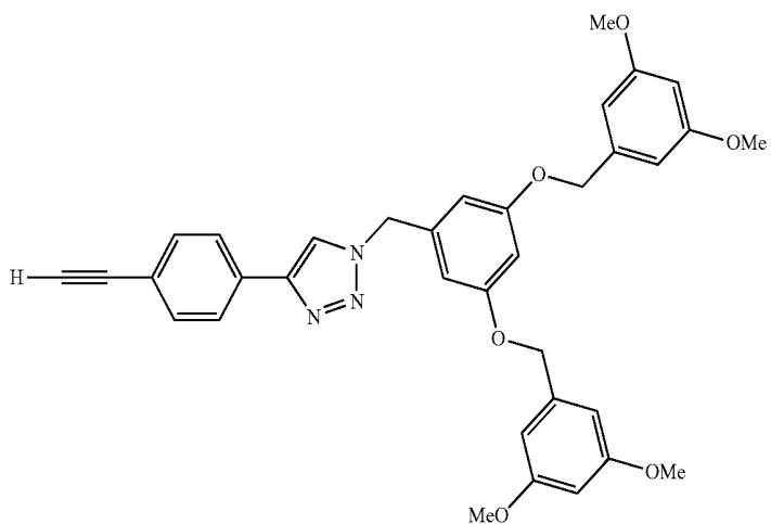
Ligand L2
